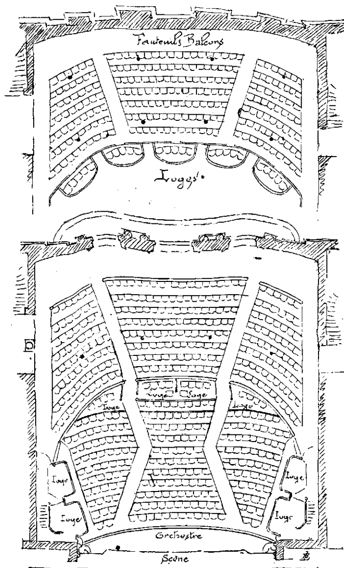
LYCÉEUM-THEATRE A ITHACA. — PLANS.
